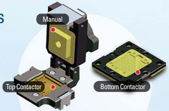
PoP Test Socket
