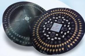
Wafer Level CSP Probe Card
